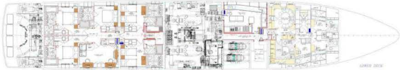
LOWER DECK
